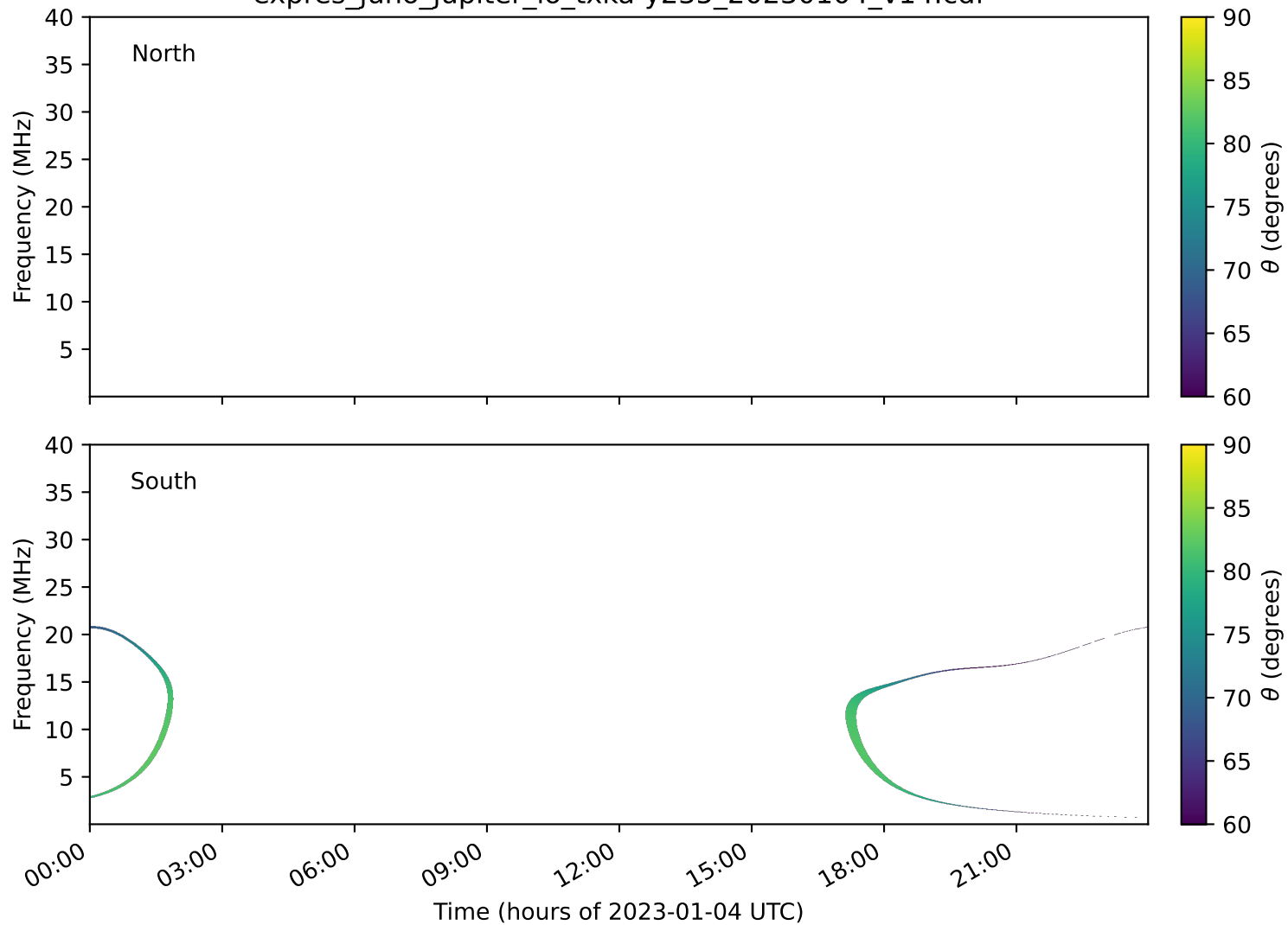
expres_juno_jupiter_io_txka-y235_20230104_v14.cdf
