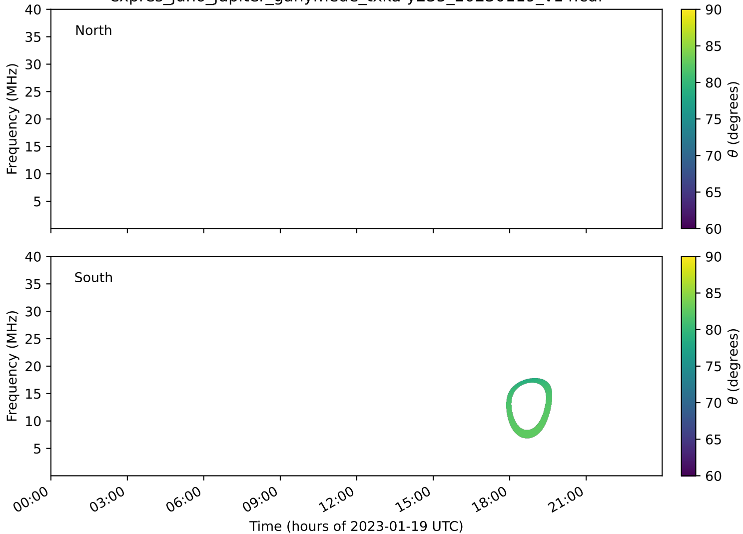
expres_juno_jupiter_ganymede_txka-y235_20230119_v14.cdf
