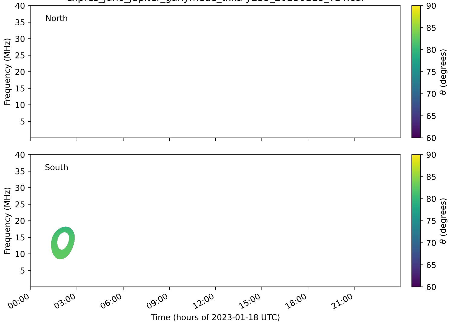
expres_juno_jupiter_ganymede_txka-y235_20230118_v14.cdf
