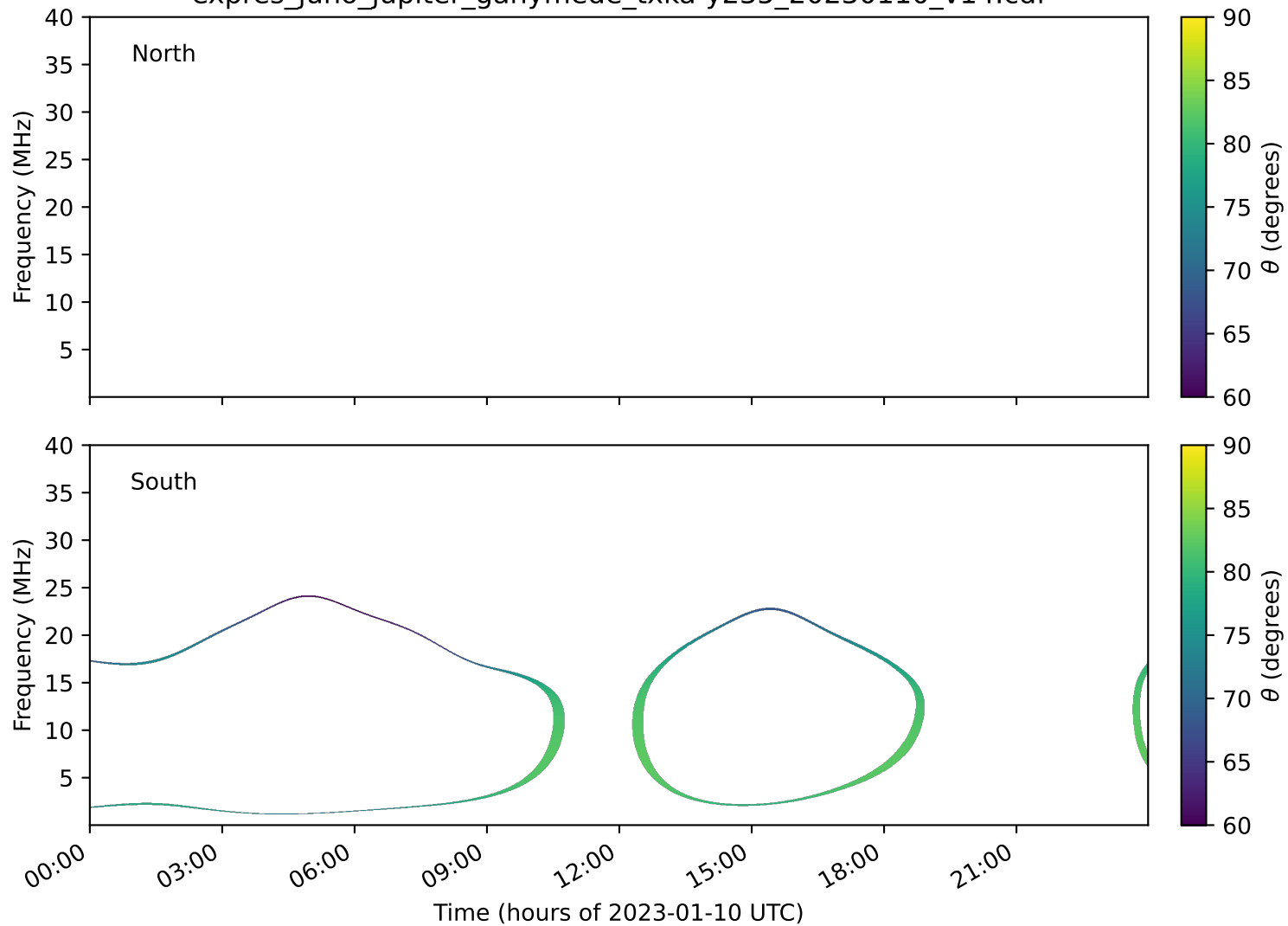
expres_juno_jupiter_ganymede_txka-y235_20230110_v14.cdf
