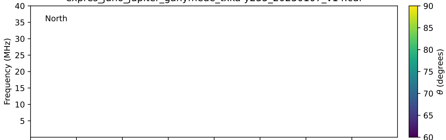
expres_juno_jupiter_ganymede_txka-y235_20230107_v14.cdf
