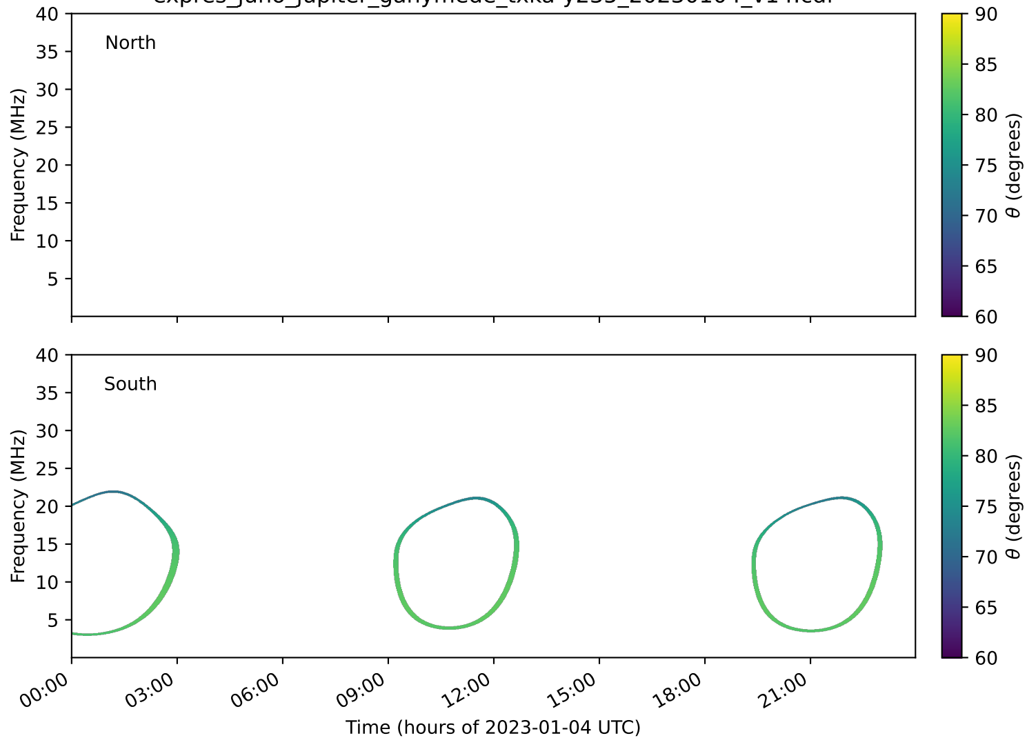
expres_juno_jupiter_ganymede_txka-y235_20230104_v14.cdf
