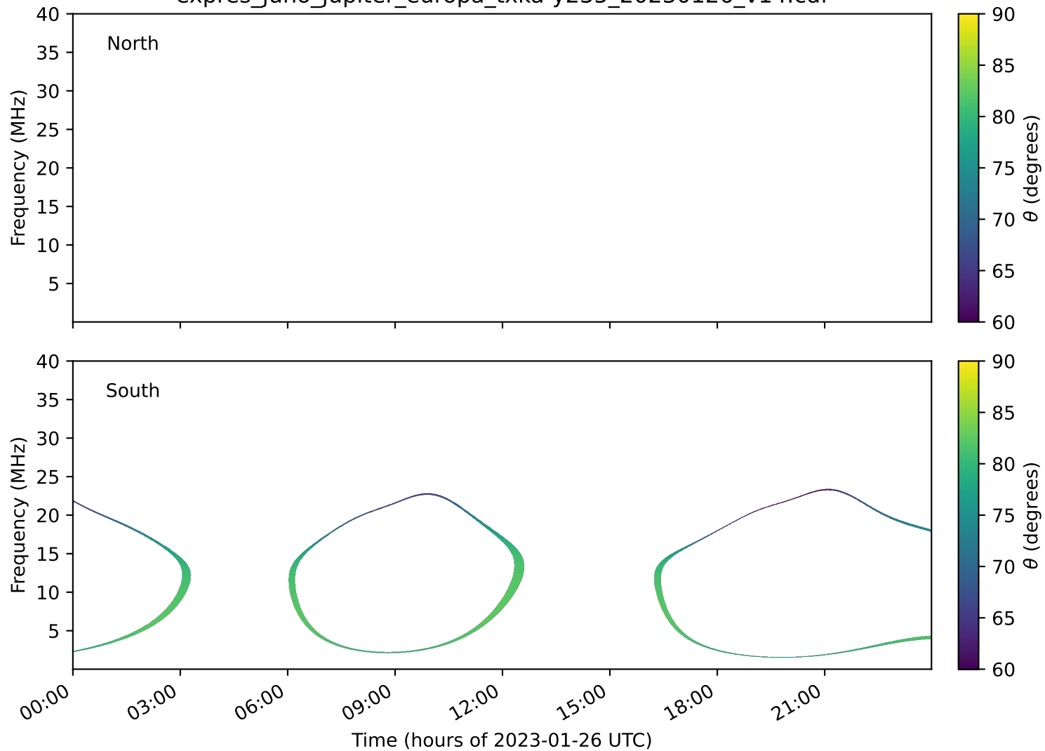
expres_juno_jupiter_europa_txka-y235_20230126_v14.cdf
