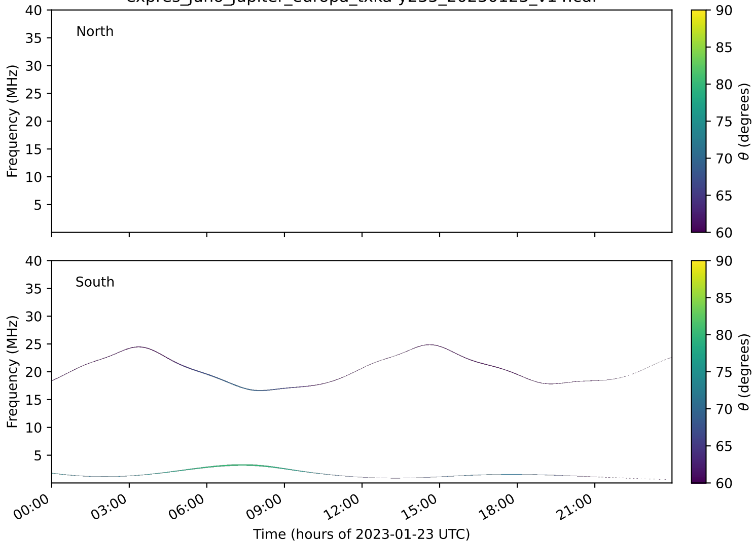
expres_juno_jupiter_europa_txka-y235_20230123_v14.cdf
