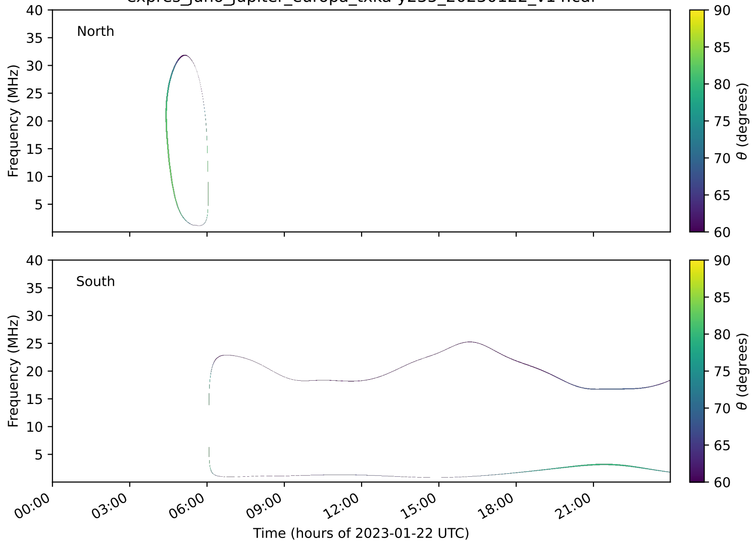
expres_juno_jupiter_europa_txka-y235_20230122_v14.cdf
