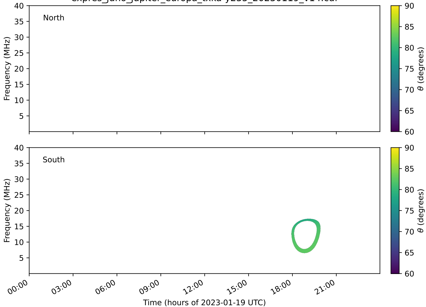
expres_juno_jupiter_europa_txka-y235_20230119_v14.cdf
