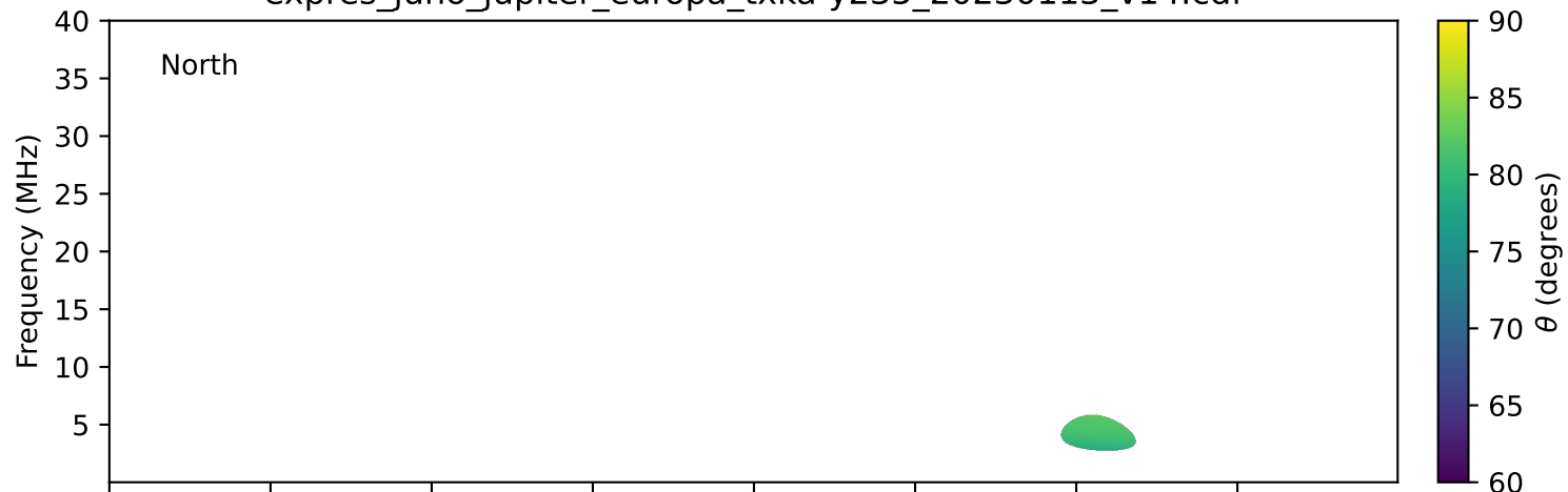
expres_juno_jupiter_europa_txka-y235_20230113_v14.cdf
