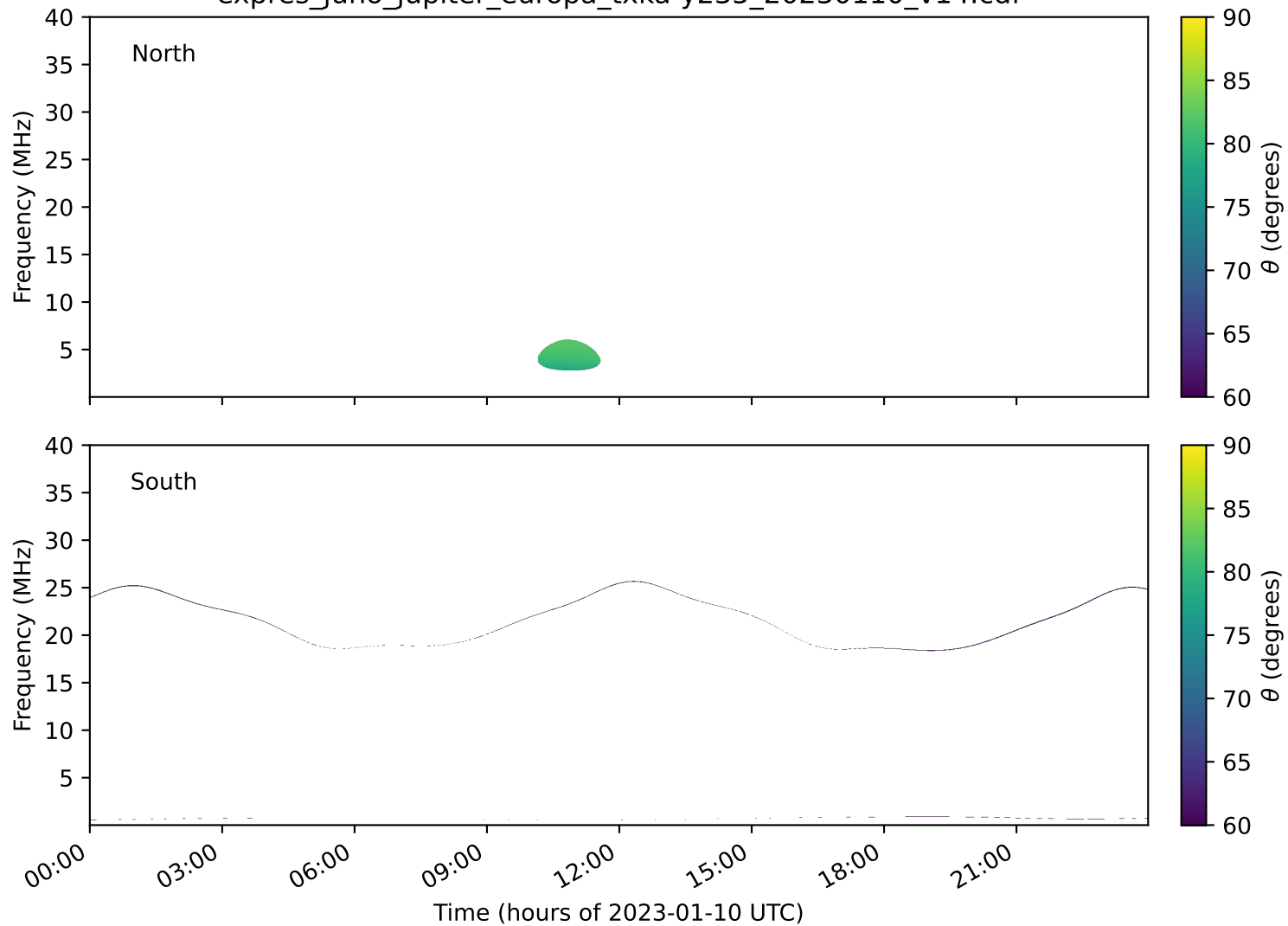
expres_juno_jupiter_europa_txka-y235_20230110_v14.cdf
