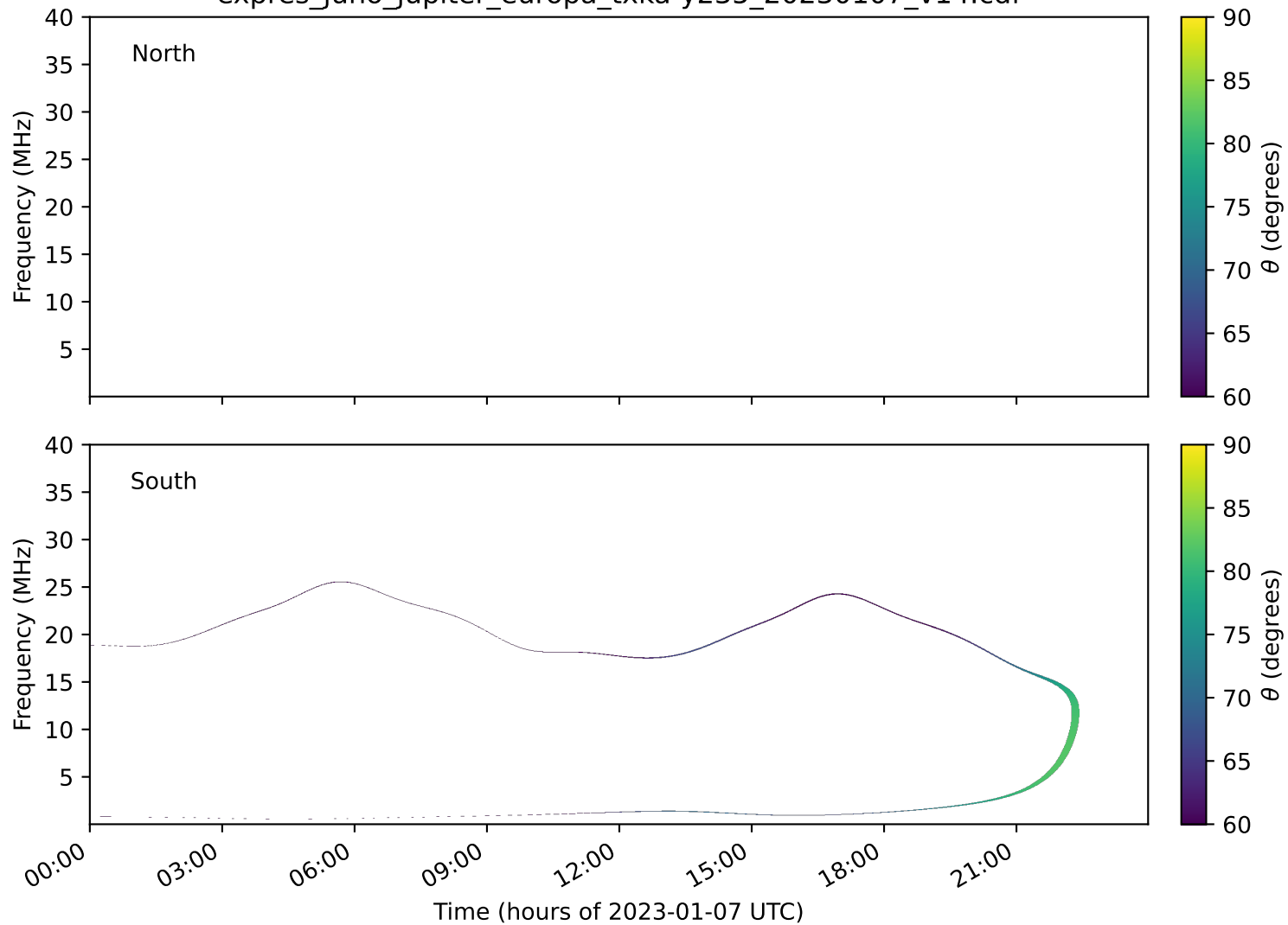
expres_juno_jupiter_europa_txka-y235_20230107_v14.cdf
