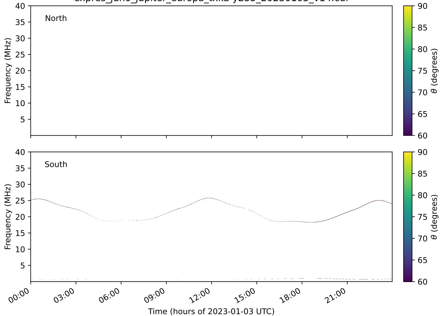
expres_juno_jupiter_europa_txka-y235_20230103_v14.cdf
