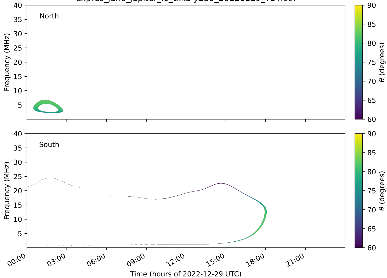
expres_juno_jupiter_io_txka-y235_20221229_v14.cdf
