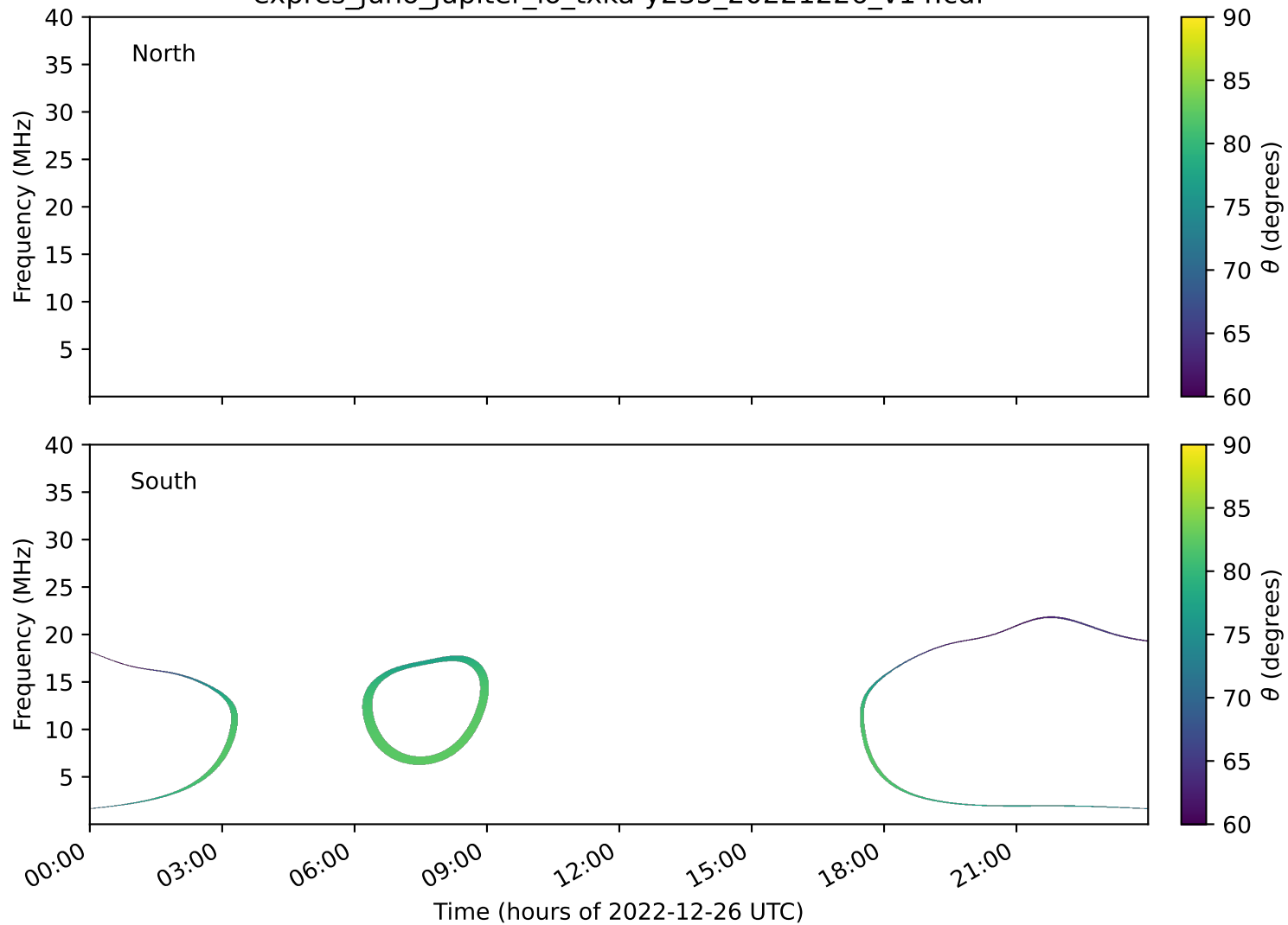
expres_juno_jupiter_io_txka-y235_20221226_v14.cdf
