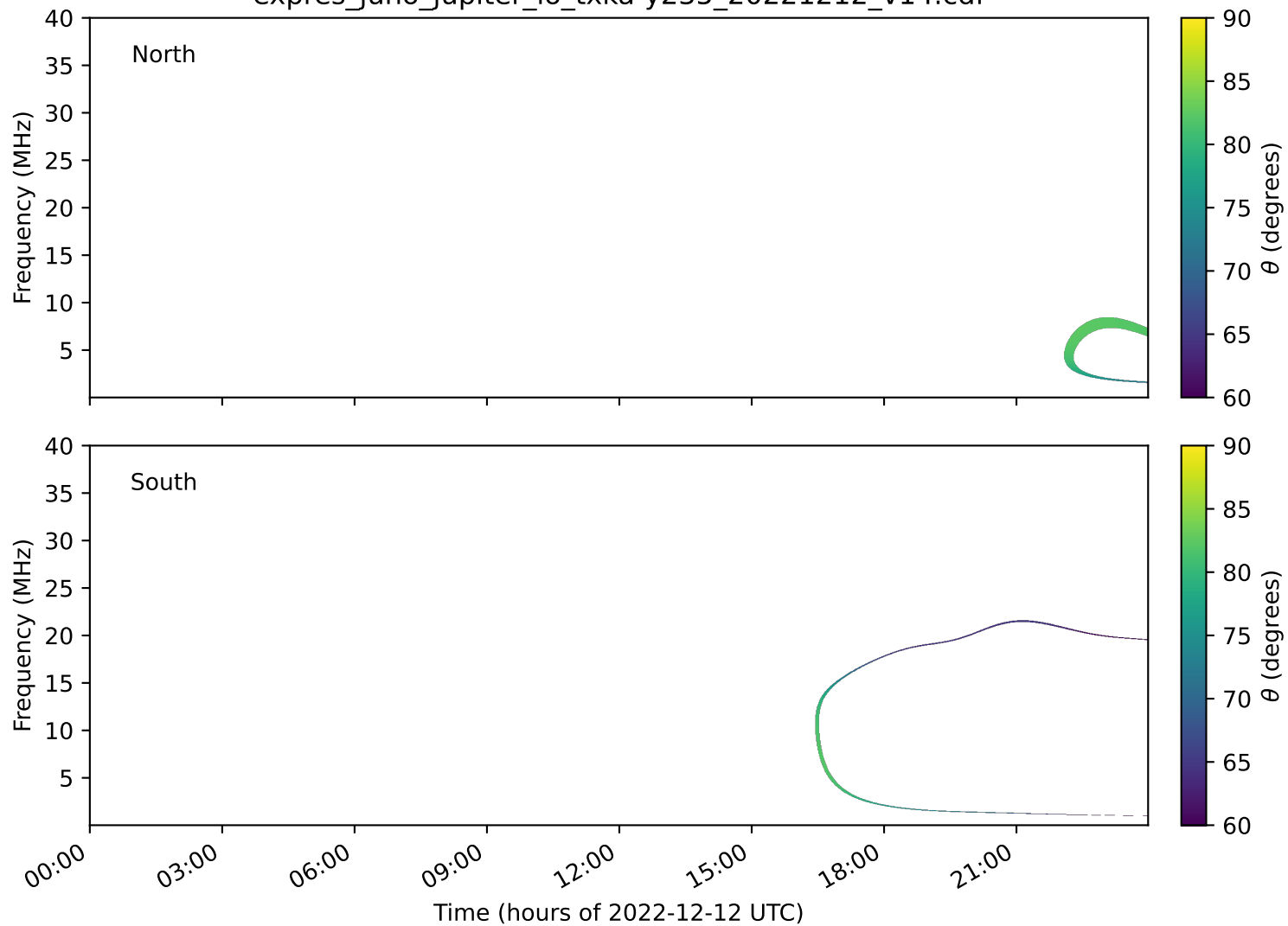
expres_juno_jupiter_io_txka-y235_20221212_v14.cdf
