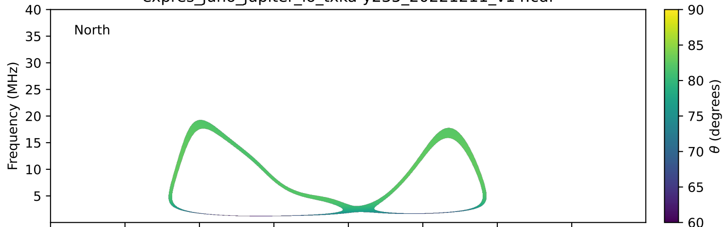
expres_juno_jupiter_io_txka-y235_20221211_v14.cdf
