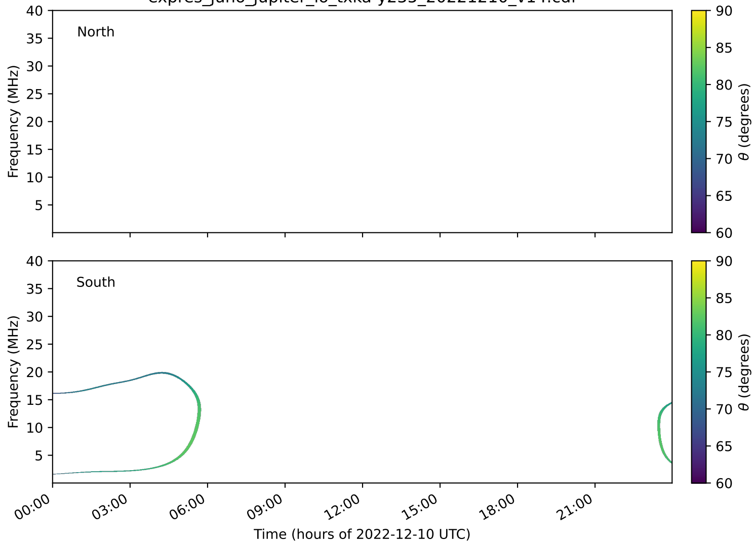
expres_juno_jupiter_io_txka-y235_20221210_v14.cdf
