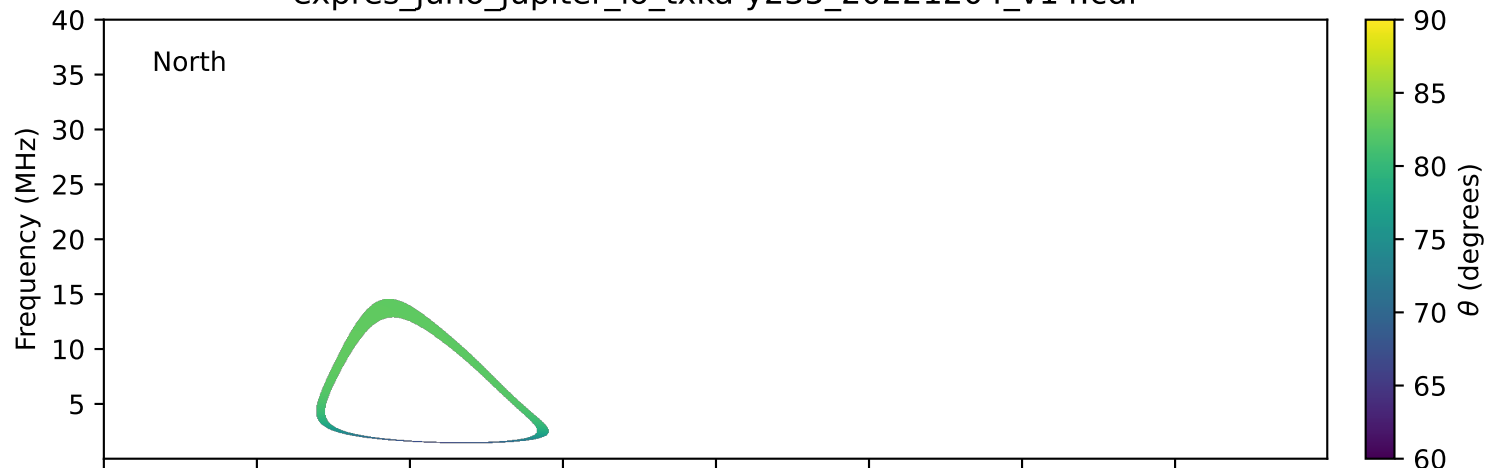
expres_juno_jupiter_io_txka-y235_20221204_v14.cdf
