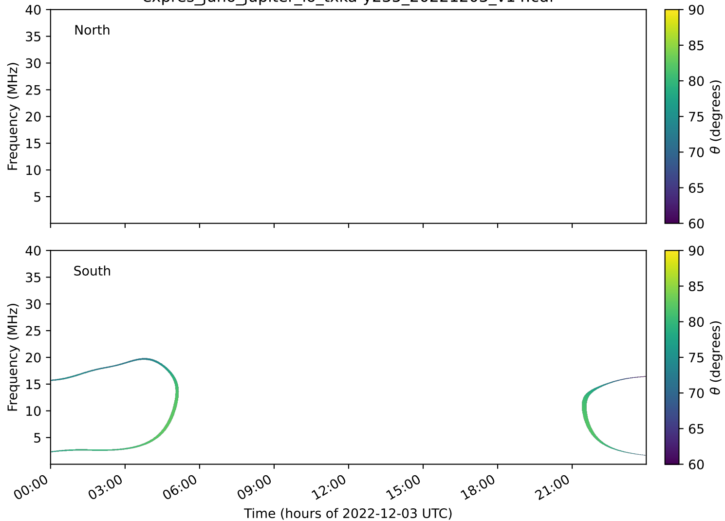
expres_juno_jupiter_io_txka-y235_20221203_v14.cdf
