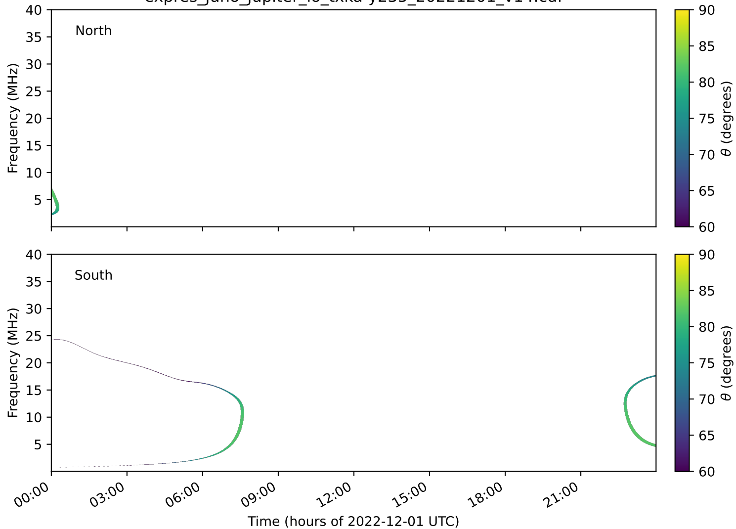
expres_juno_jupiter_io_txka-y235_20221201_v14.cdf
