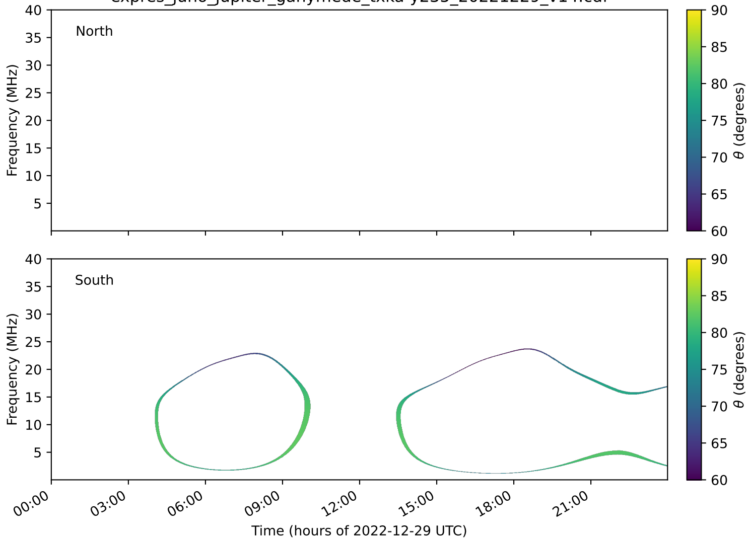
expres_juno_jupiter_ganymede_txka-y235_20221229_v14.cdf
