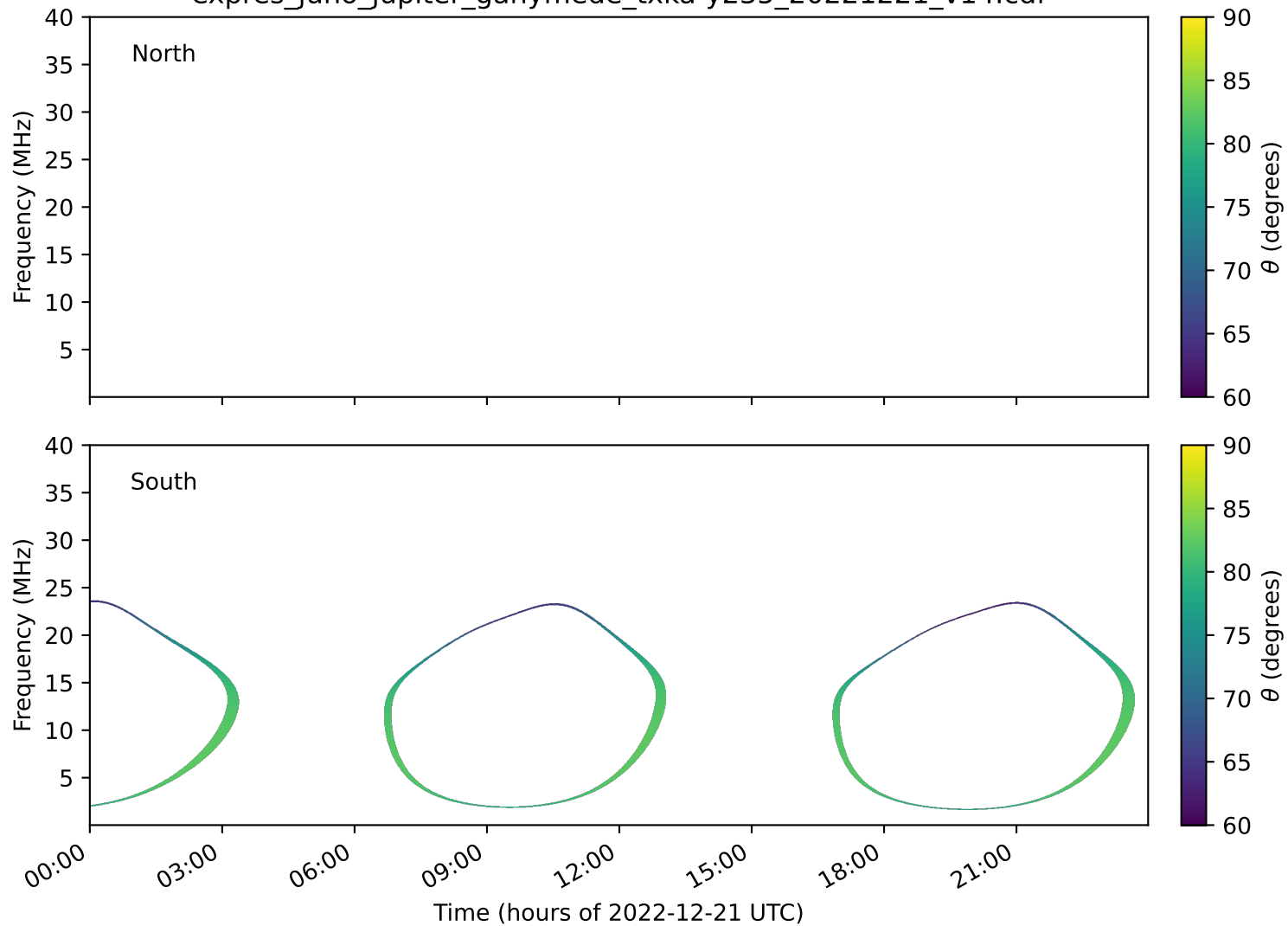
expres_juno_jupiter_ganymede_txka-y235_20221221_v14.cdf
