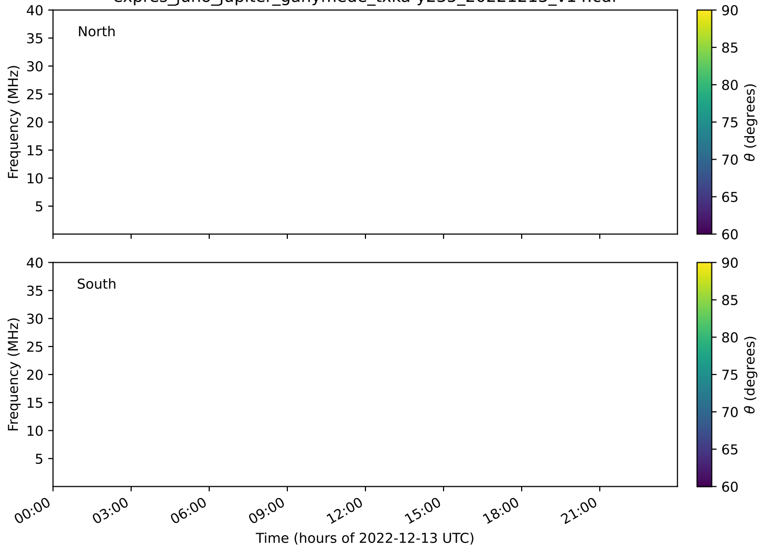
expres_juno_jupiter_ganymede_txka-y235_20221213_v14.cdf
