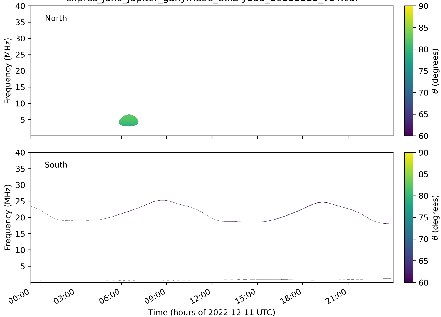
expres_juno_jupiter_ganymede_txka-y235_20221211_v14.cdf
