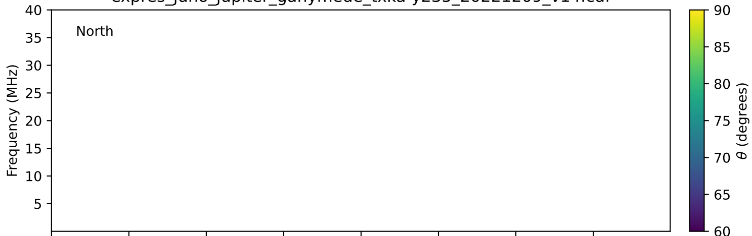
expres_juno_jupiter_ganymede_txka-y235_20221209_v14.cdf
