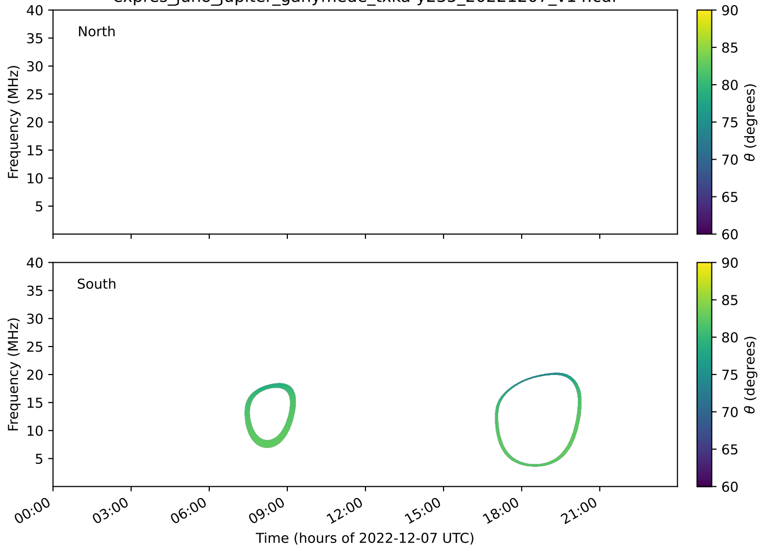
expres_juno_jupiter_ganymede_txka-y235_20221207_v14.cdf
