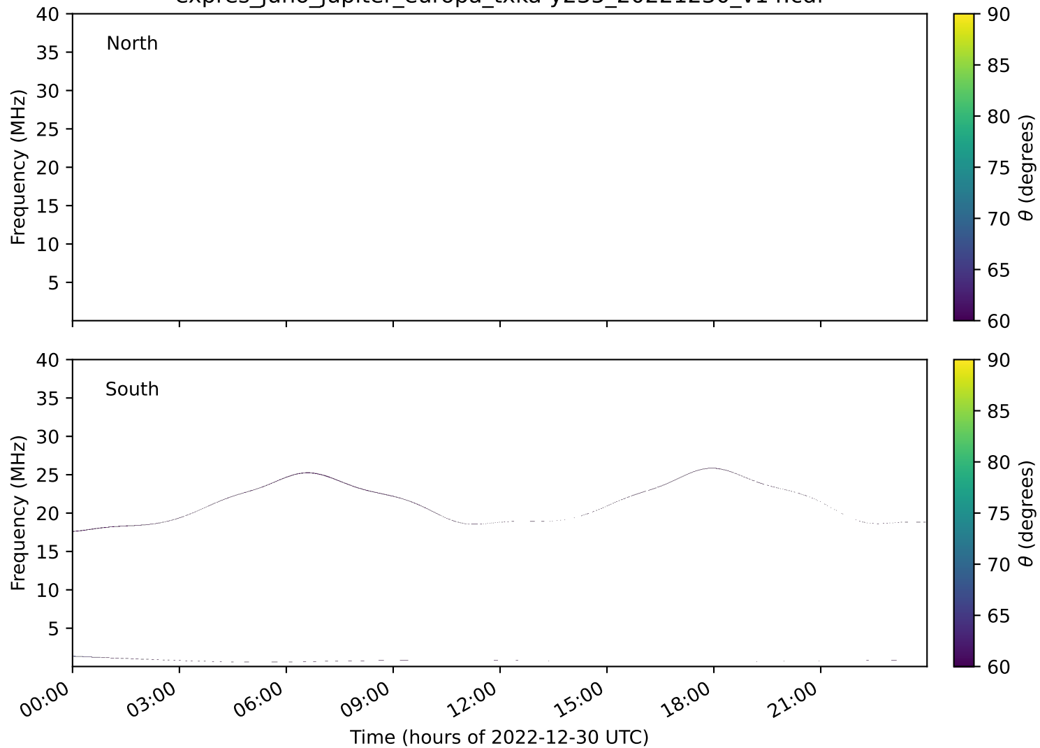
expres_juno_jupiter_europa_txka-y235_20221230_v14.cdf
