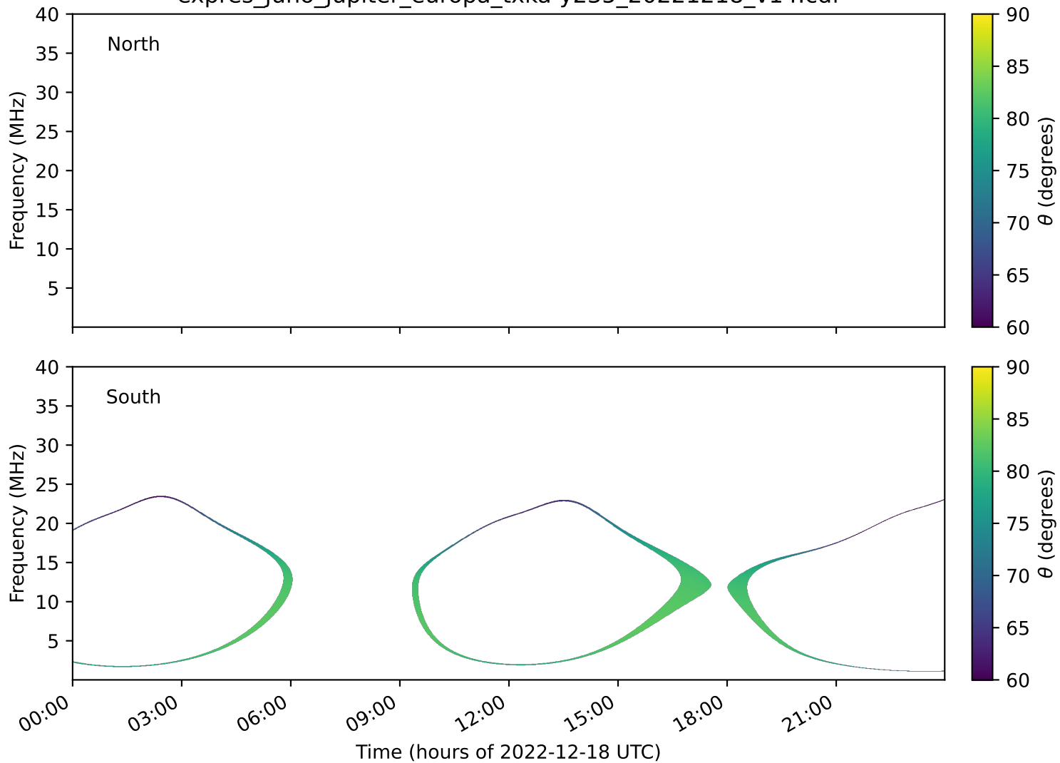
expres_juno_jupiter_europa_txka-y235_20221218_v14.cdf
