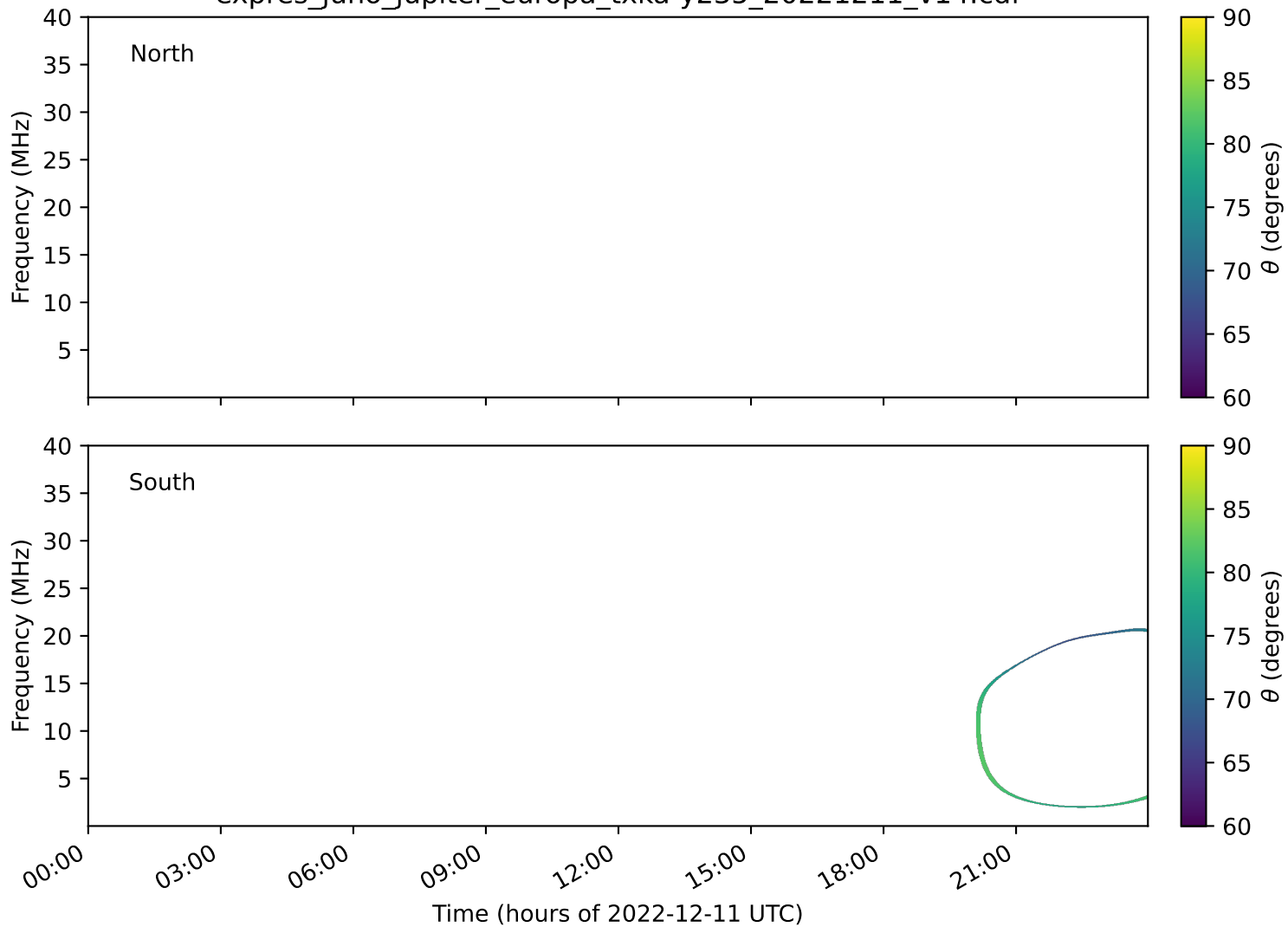
expres_juno_jupiter_europa_txka-y235_20221211_v14.cdf
