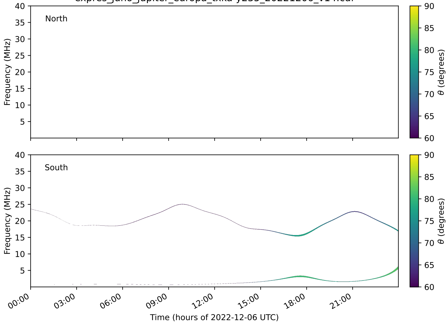
expres_juno_jupiter_europa_txka-y235_20221206_v14.cdf
