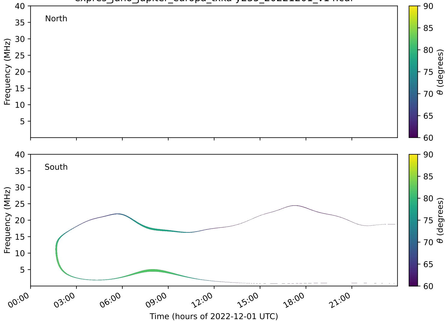
expres_juno_jupiter_europa_txka-y235_20221201_v14.cdf
