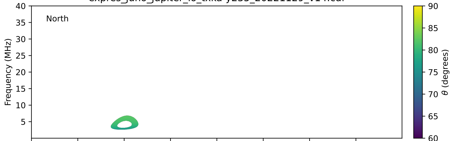
expres_juno_jupiter_io_txka-y235_20221129_v14.cdf
