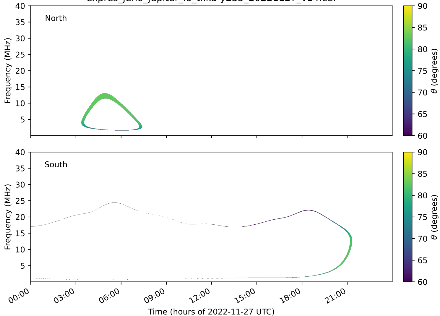
expres_juno_jupiter_io_txka-y235_20221127_v14.cdf
