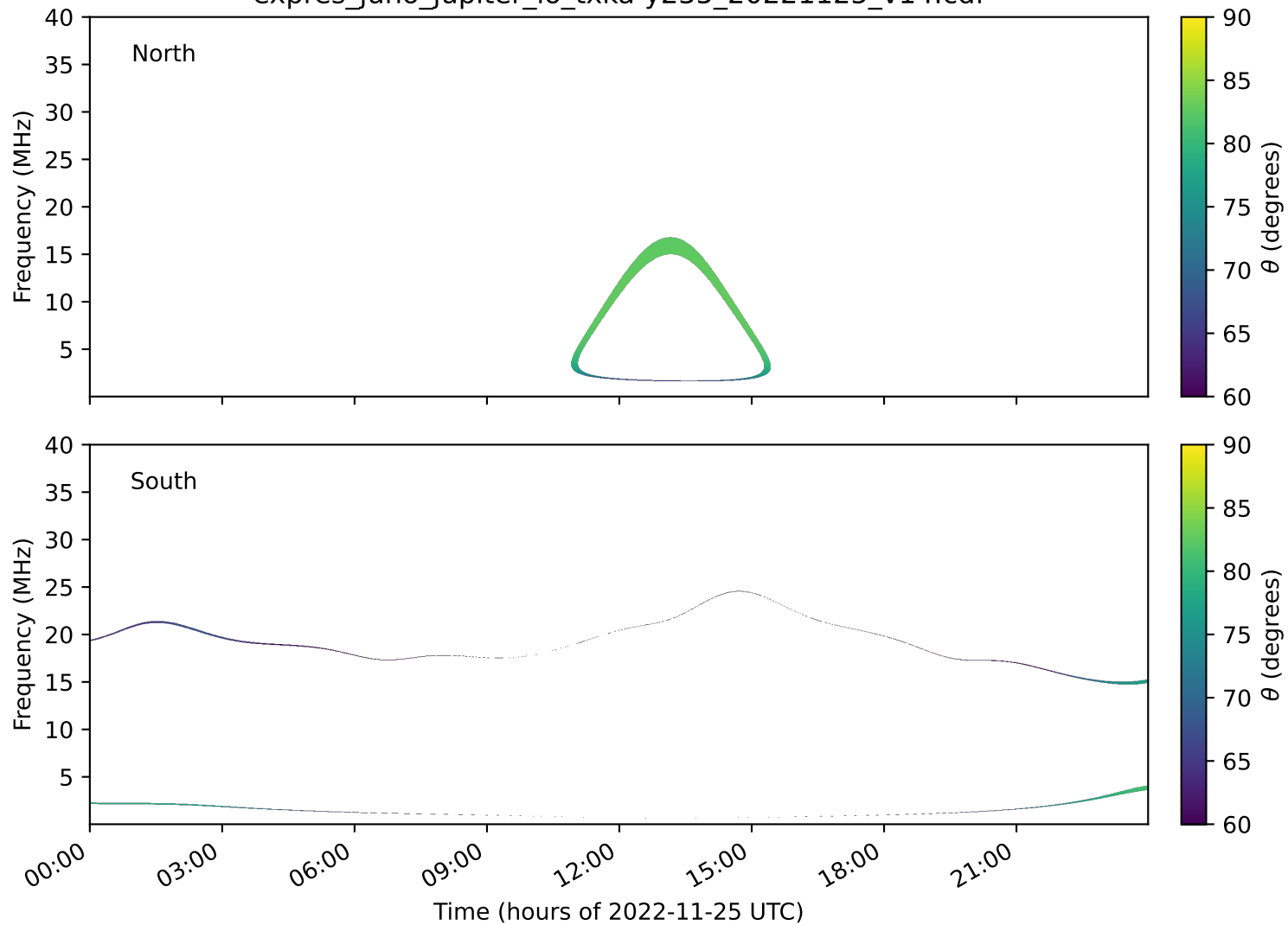
expres_juno_jupiter_io_txka-y235_20221125_v14.cdf
