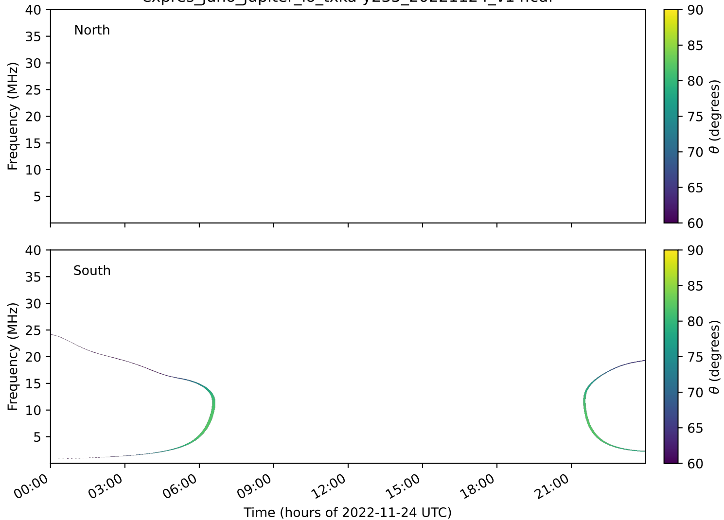
expres_juno_jupiter_io_txka-y235_20221124_v14.cdf
