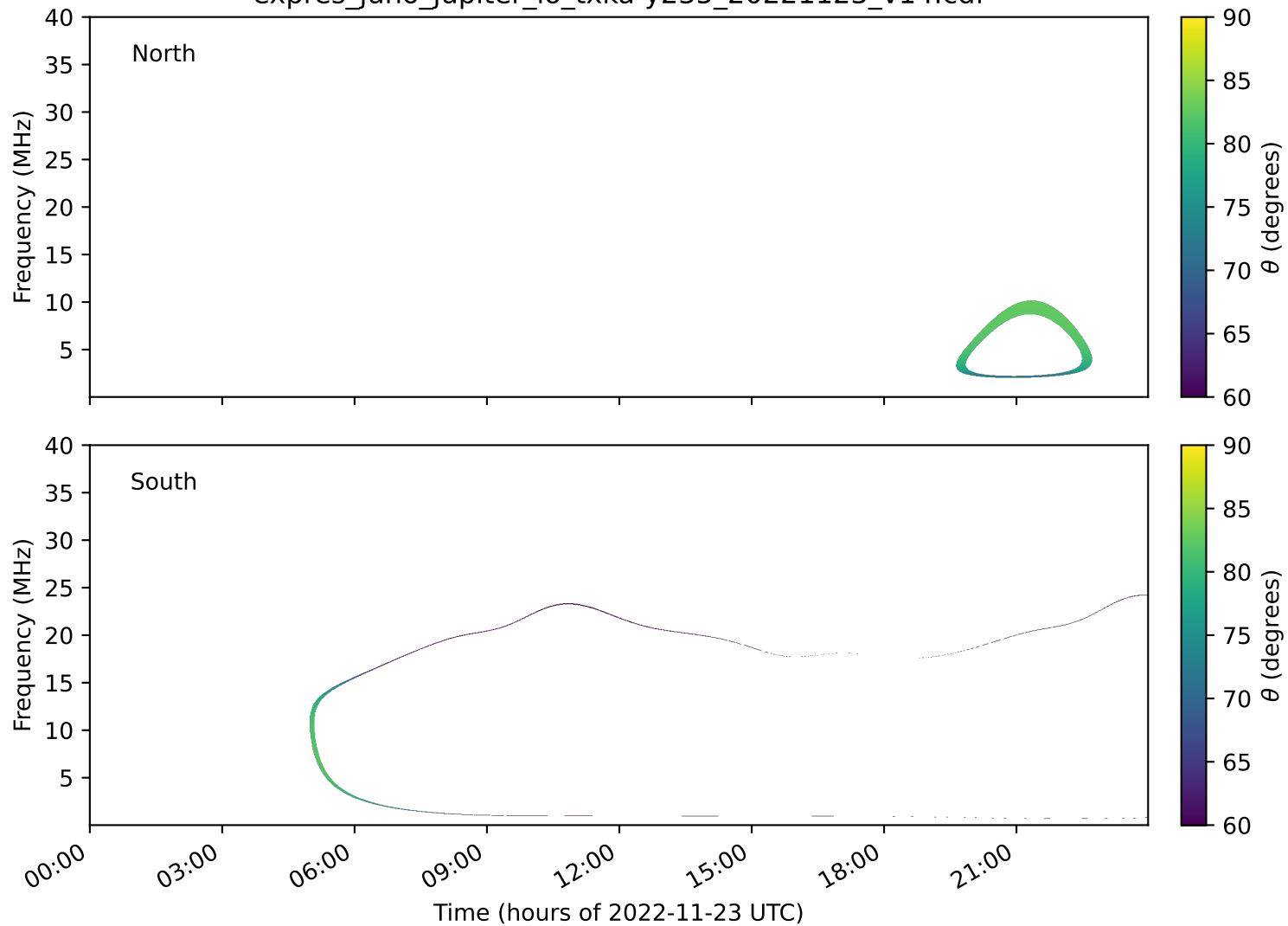
expres_juno_jupiter_io_txka-y235_20221123_v14.cdf
