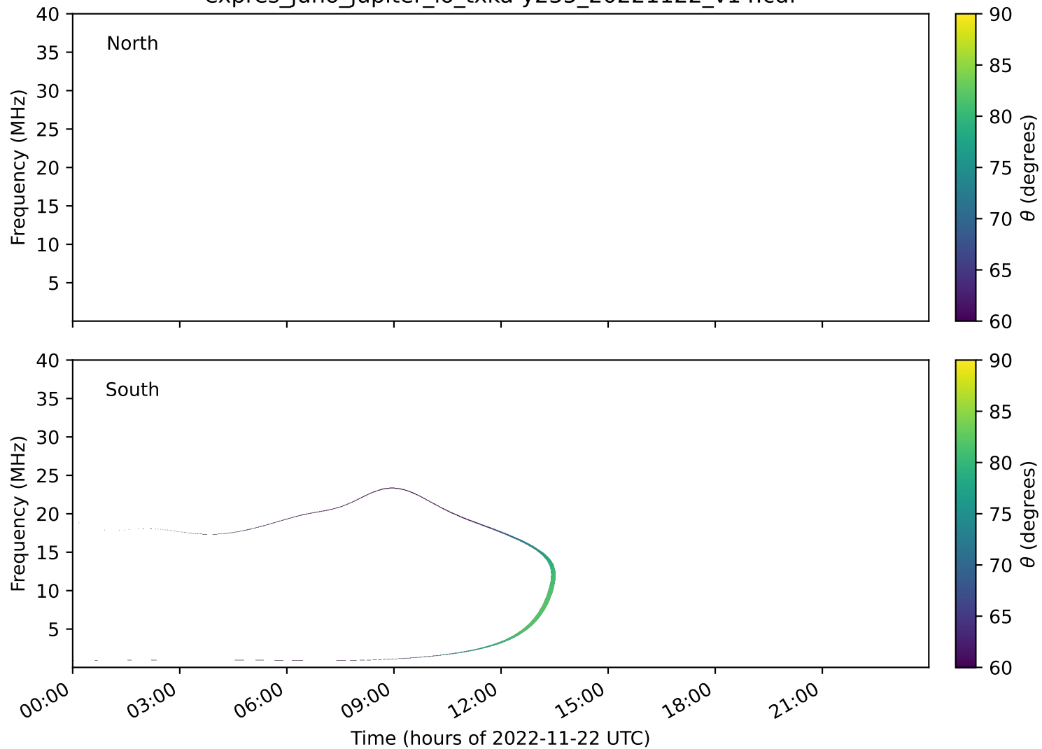
expres_juno_jupiter_io_txka-y235_20221122_v14.cdf
