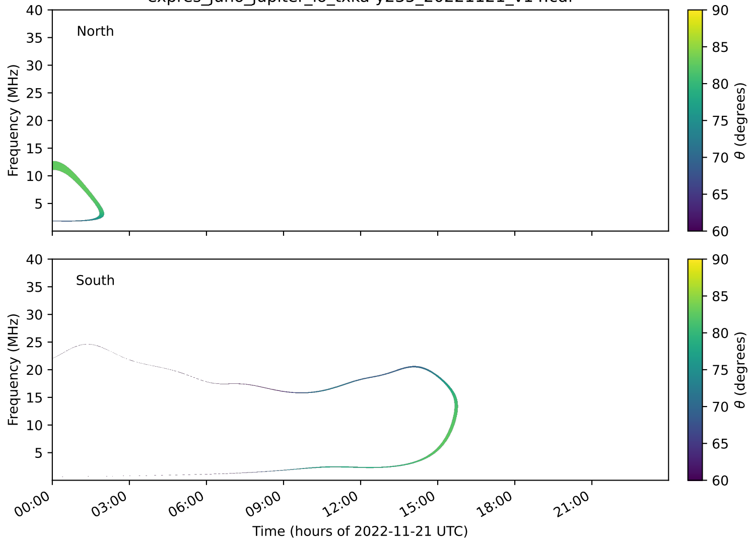
expres_juno_jupiter_io_txka-y235_20221121_v14.cdf
