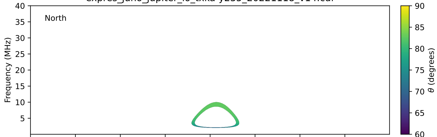
expres_juno_jupiter_io_txka-y235_20221118_v14.cdf
