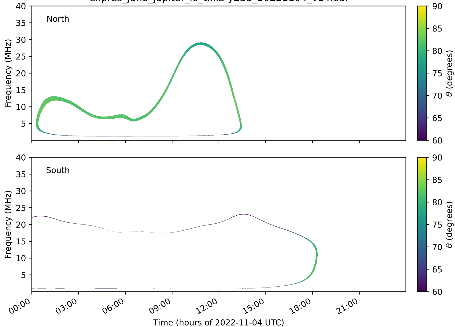
expres_juno_jupiter_io_txka-y235_20221104_v14.cdf
