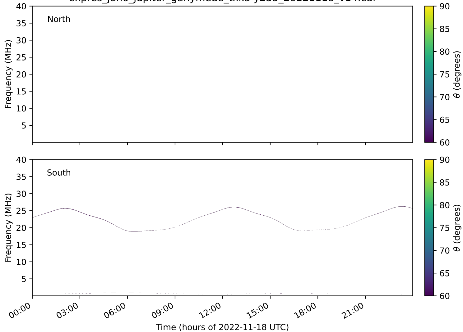
expres_juno_jupiter_ganymede_txka-y235_20221118_v14.cdf
