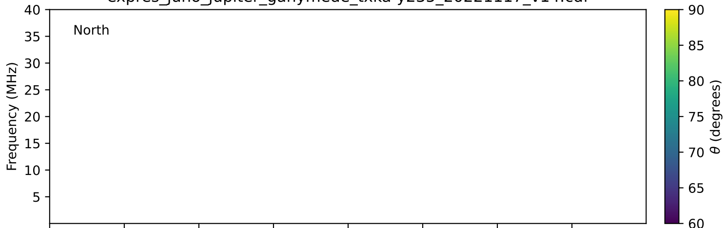
expres_juno_jupiter_ganymede_txka-y235_20221117_v14.cdf
