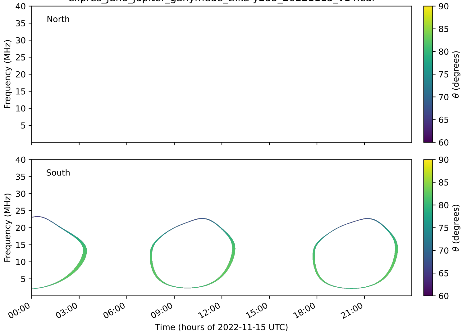
expres_juno_jupiter_ganymede_txka-y235_20221115_v14.cdf
