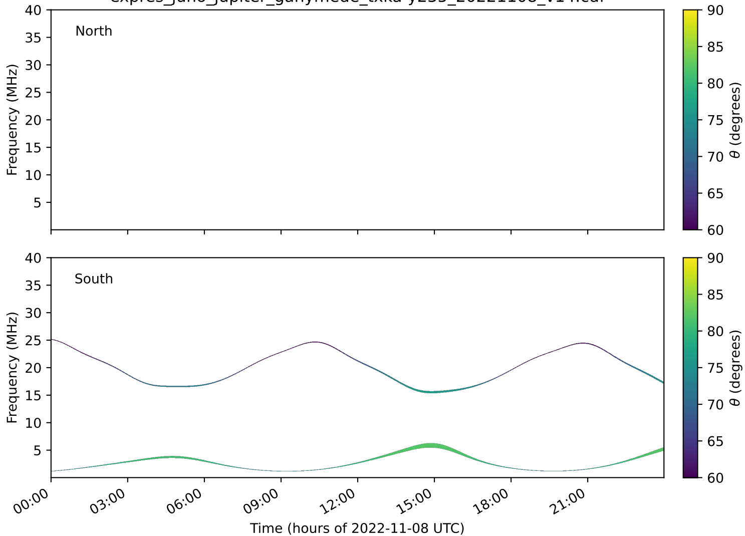
expres_juno_jupiter_ganymede_txka-y235_20221108_v14.cdf
