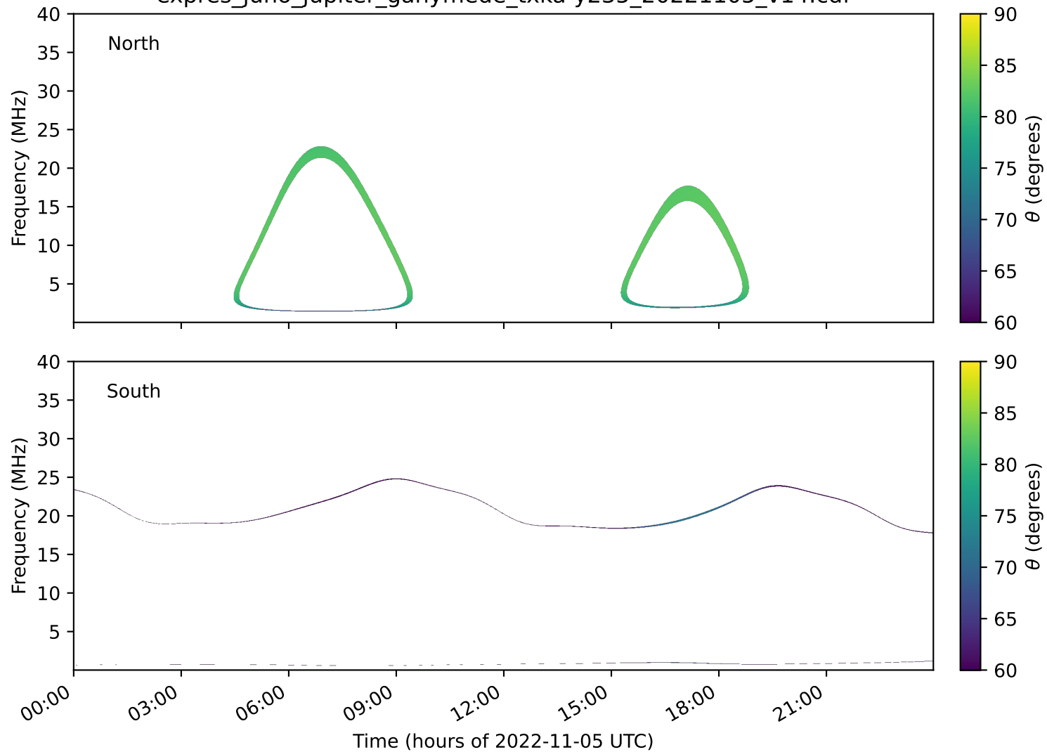
expres_juno_jupiter_ganymede_txka-y235_20221105_v14.cdf
