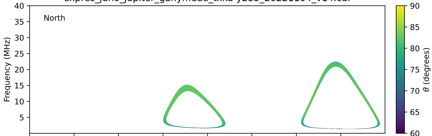
expres_juno_jupiter_ganymede_txka-y235_20221104_v14.cdf
