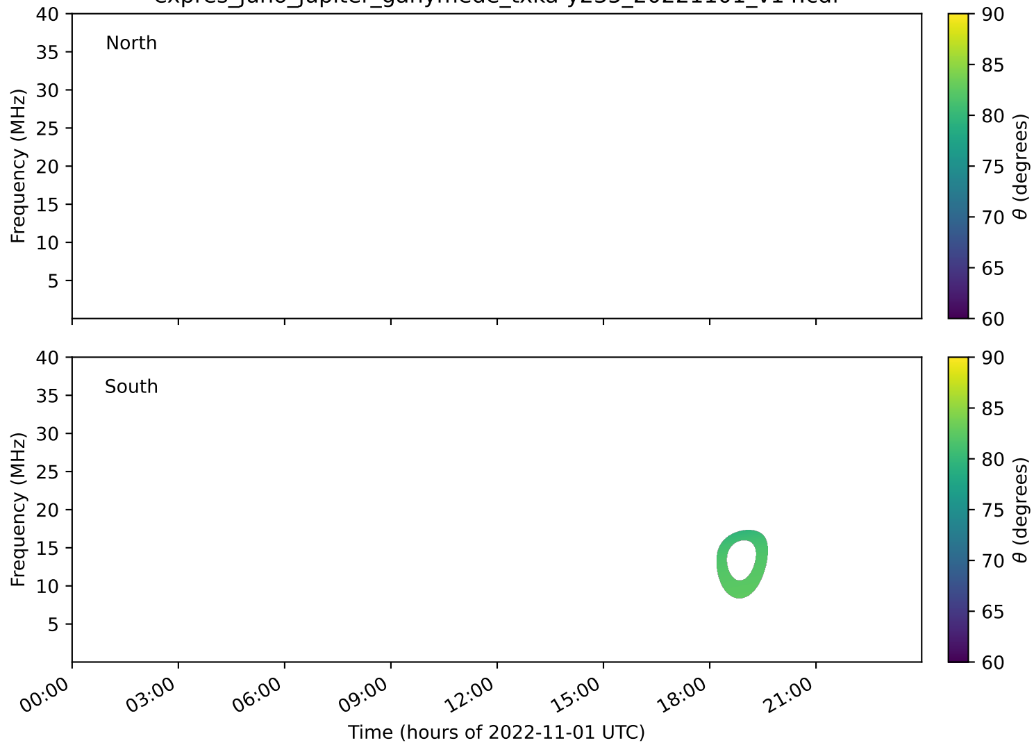
expres_juno_jupiter_ganymede_txka-y235_20221101_v14.cdf
