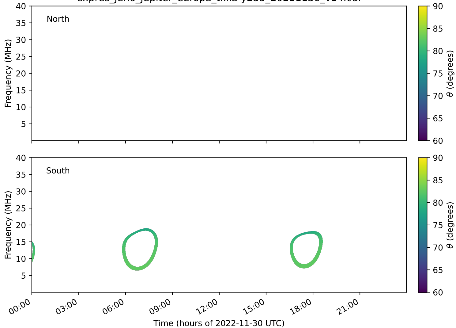
expres_juno_jupiter_europa_txka-y235_20221130_v14.cdf
